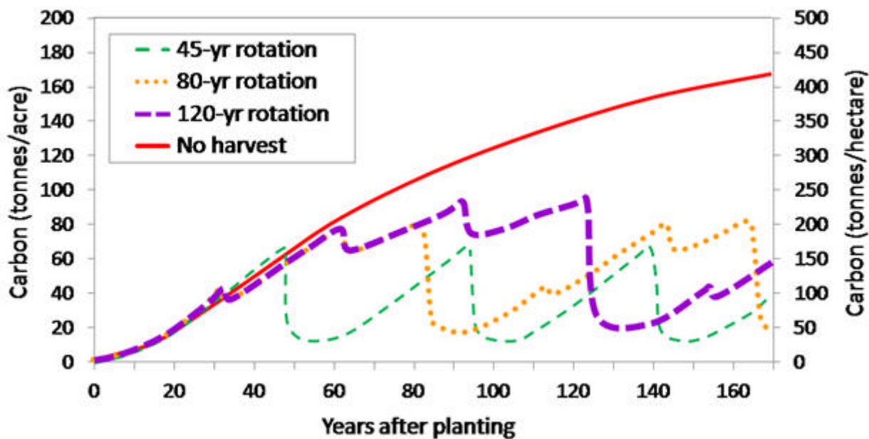
Figure 1. Carbon storage in the forest pool for 45 , 80 , 120 year rotations or harvest cycles and no harvest option that should be considered a potential maximum for carbon storage in the forest pool.
