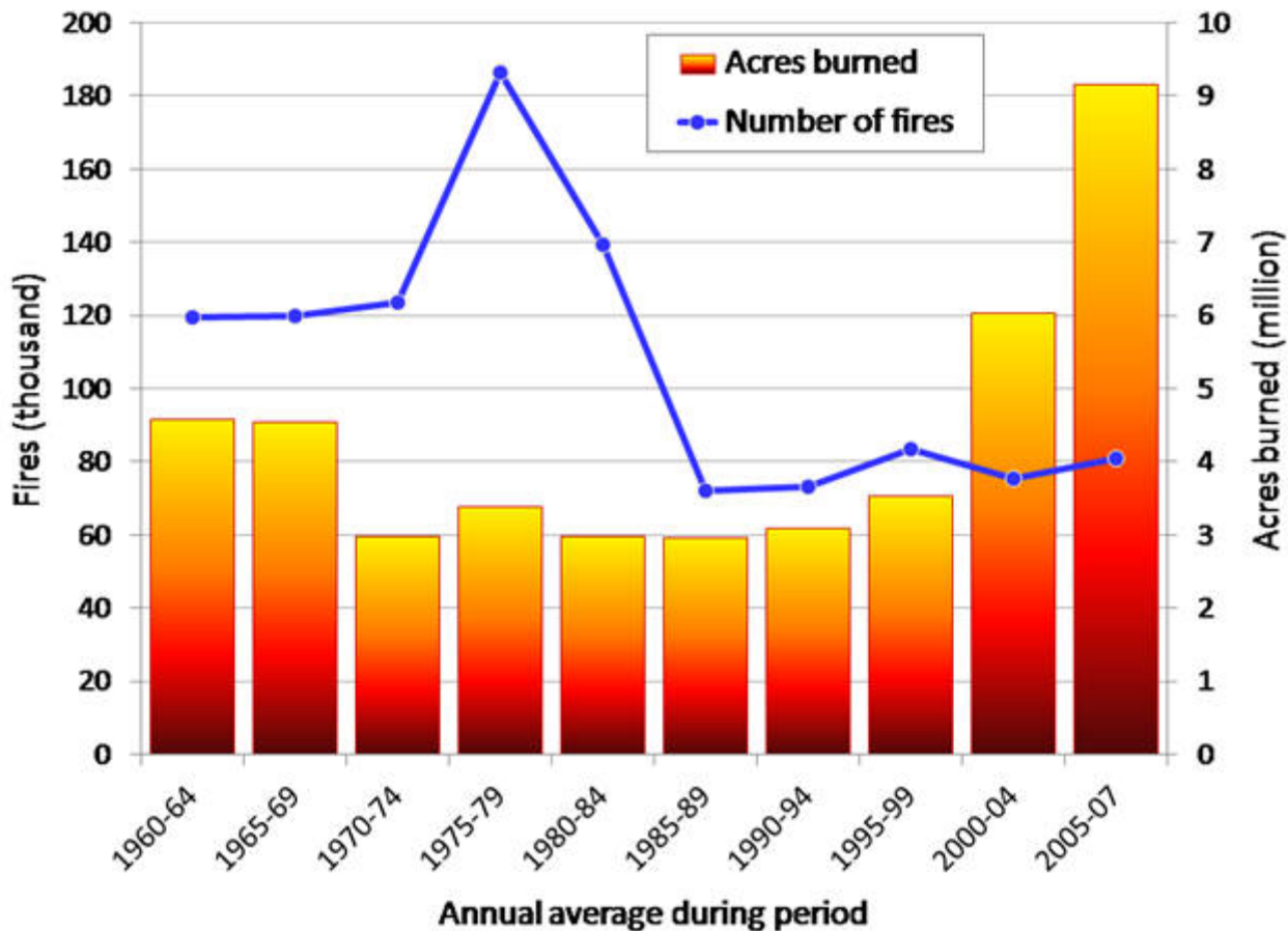
Figure 3. Wildfires in U.S., acres burned and number of fires, 1960–2007.
